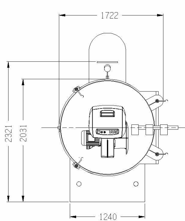
DETAIL: FRONT ELEVATION
